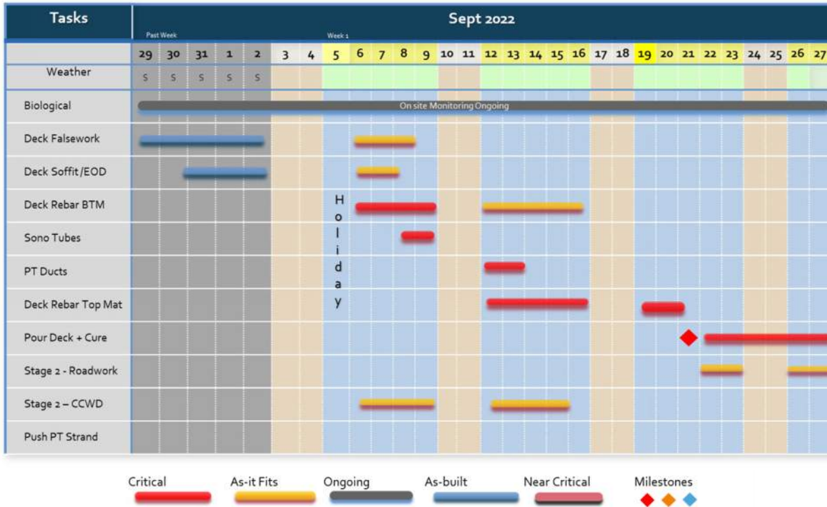
Figure 1 – Weekly Look-ahead Schedule
